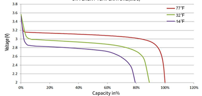
CELL DISCHARGE CURVES UNDER DIFFERENT TEMPERATURE(0.5C)
