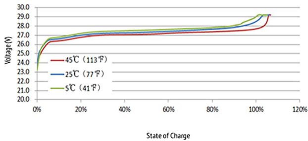
CHARGE VOLTAGE CHARACTERISTICS at VARIOUS TEMPERATURES CHARGE 0.2C
